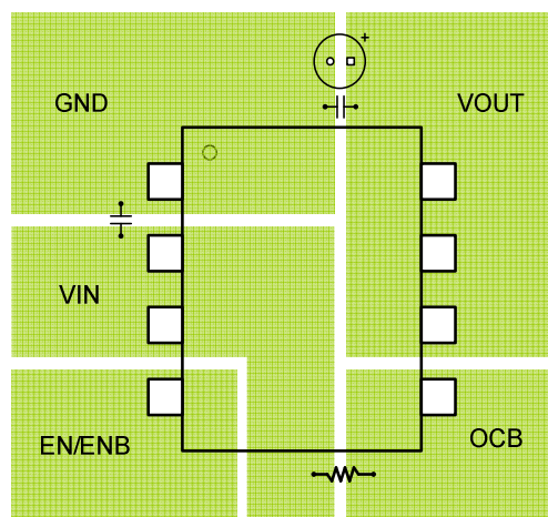
PCB Layout Guide (SO8)
