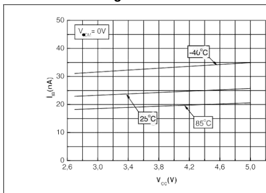
Figure 5. Input bias current versus supply voltage
