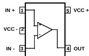
Pin connections (top view)
