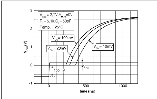
Figure 9. Response time versus overdrive with positive transition
