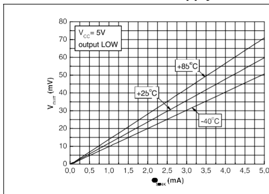
Figure 3. Output voltage versus output current at 5 V supply
