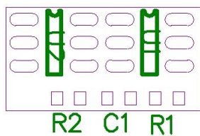
TOP SILKSCREEN
