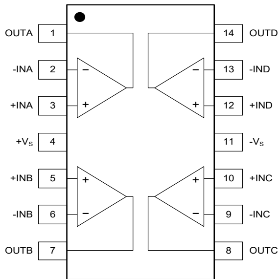
TSSOP-14/SOIC-14
