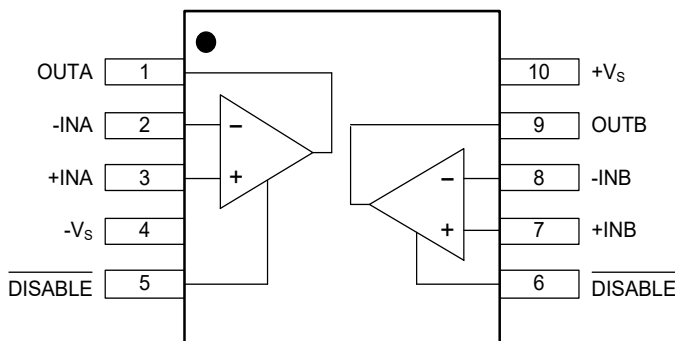
MSOP-10
