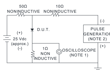
FIG.6-TEST CIRCUIT DIAGRAM AND REVERSE RECOVERY TIME CHARACTERISTIC
