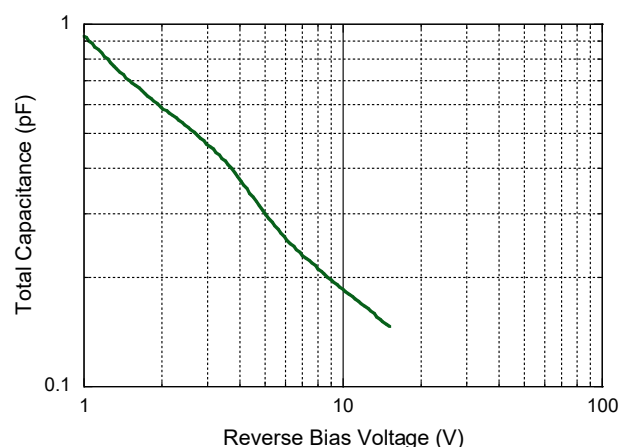
Capacitance vs. Voltage Gamma = 1.00 \pm 10\% (2 - 12 V)
